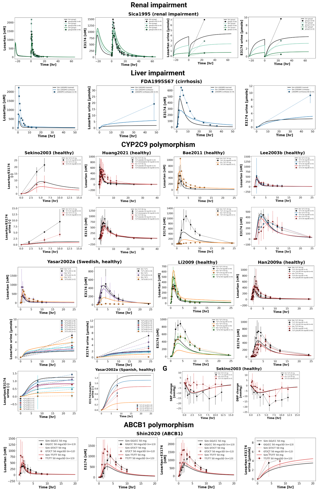
Figure 3. Reproduction of study simulations (renal and liver impairment, CYP2C9 and ABCB1 polymorphism) from the primary publication. Data is taken from (Bae et al., 2011; FDA, 1995b; Han et al., 2009; Huang et al., 2021; Lee et al., 2003; Li et al., 2009; Sekino et al., 2003; Shin et al., 2020; Sica et al., 1995; Yasar et al., 2002a).
