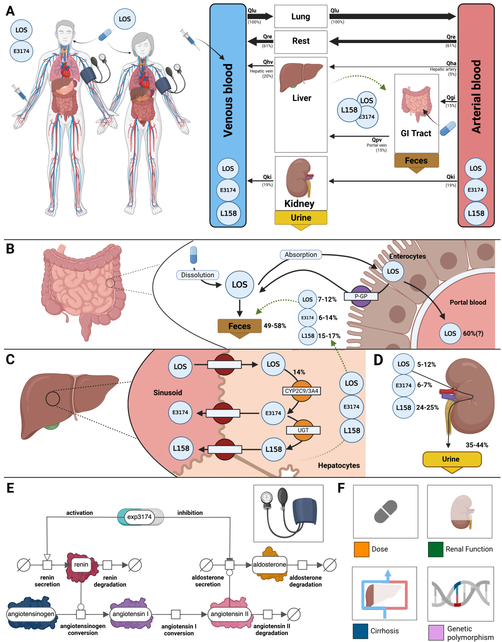
Figure 1. Whole-body PBPK/PD model of losartan.
